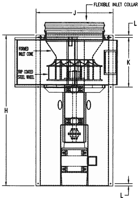
TOP VIEW
