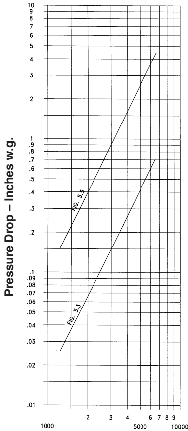
Model 912 Damper size 12" Dia. Velocity vs. Pressure Drop
