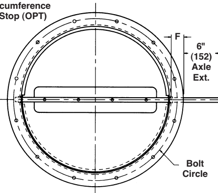
Illustrated with Optional Bolt Holes (OPT) (Face View)
