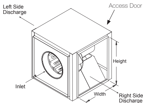
BSQ-M Side Discharge Duct Openings
