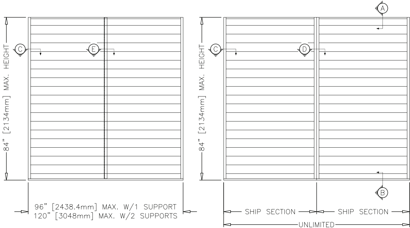
SINGLE SECTION W/ SUPPORT ANGLES
