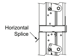
Horizontal Mullion (standard)
