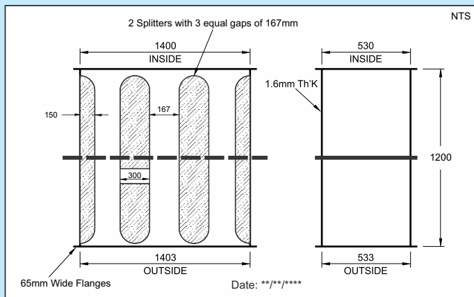
Sketch Of The Selected Silencer
