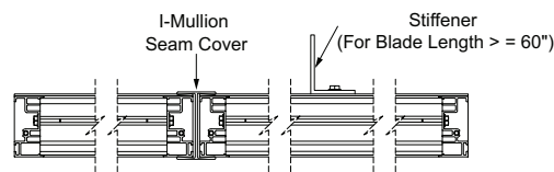
Visible Vertical Mullion (standard)
