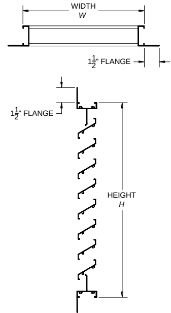
MODEL: 2215 FRAME: FLANGE FRAME FLANGE-MOUNT (FM)
