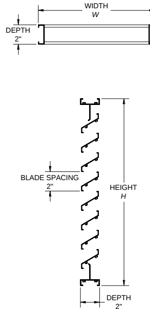
MODEL: 2210 FRAME: CHANNEL FRAME DUCT-MOUNT (DM)
