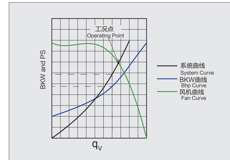
Fig.4 Operating Point
