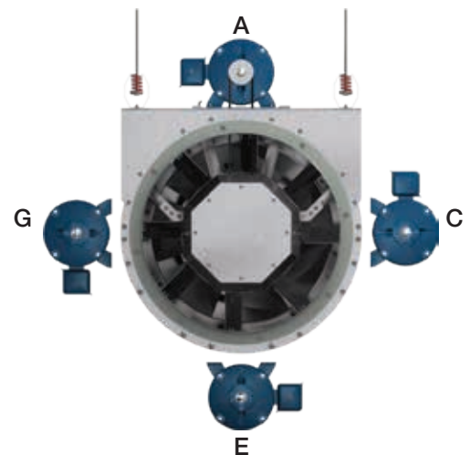
Multiple Motor Positions
