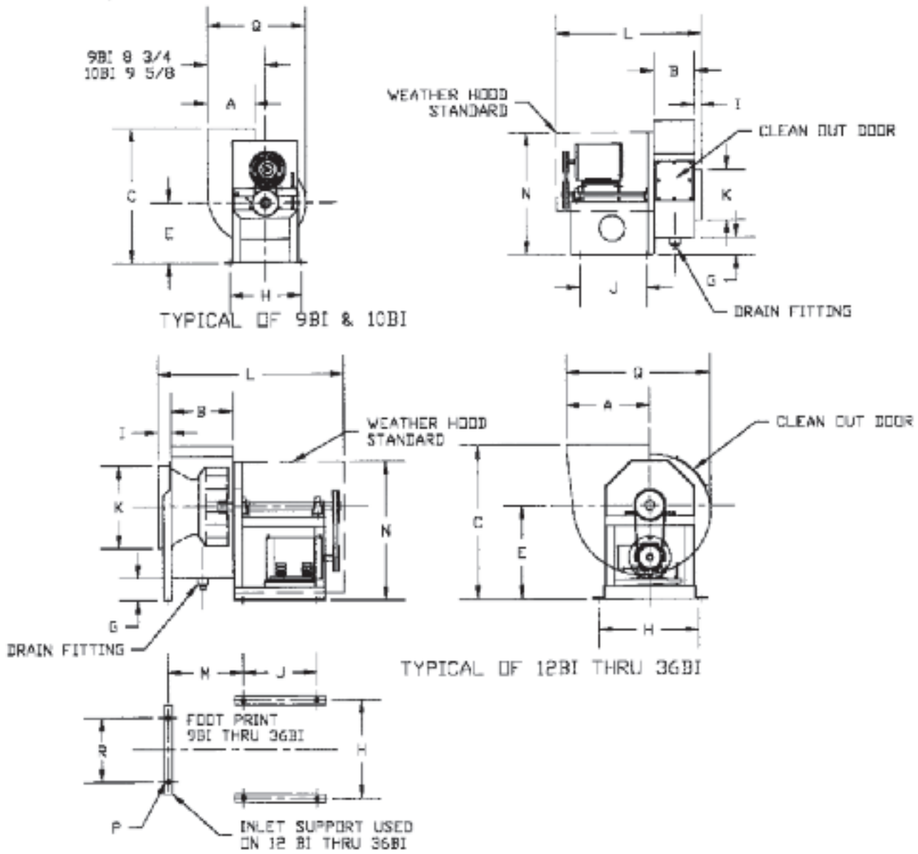
Dimensional Table
