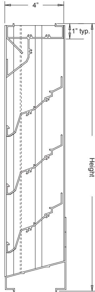
Section View
