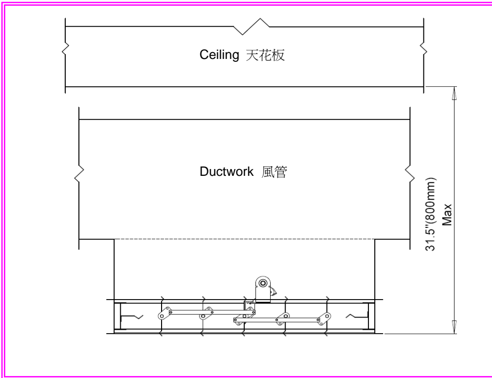
Horizontal installation
