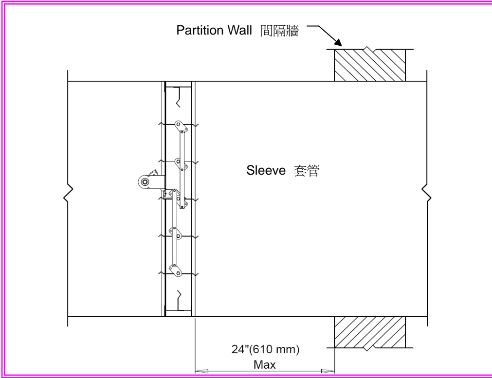
Vertical installation
