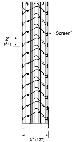
Vertical Section
