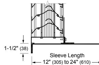
Sleeve (optional)
