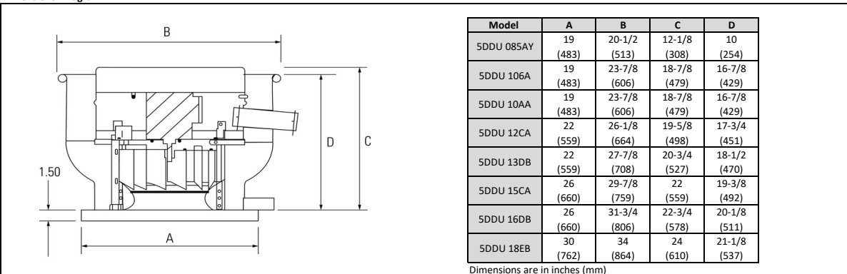
Dimensional Diagram:
