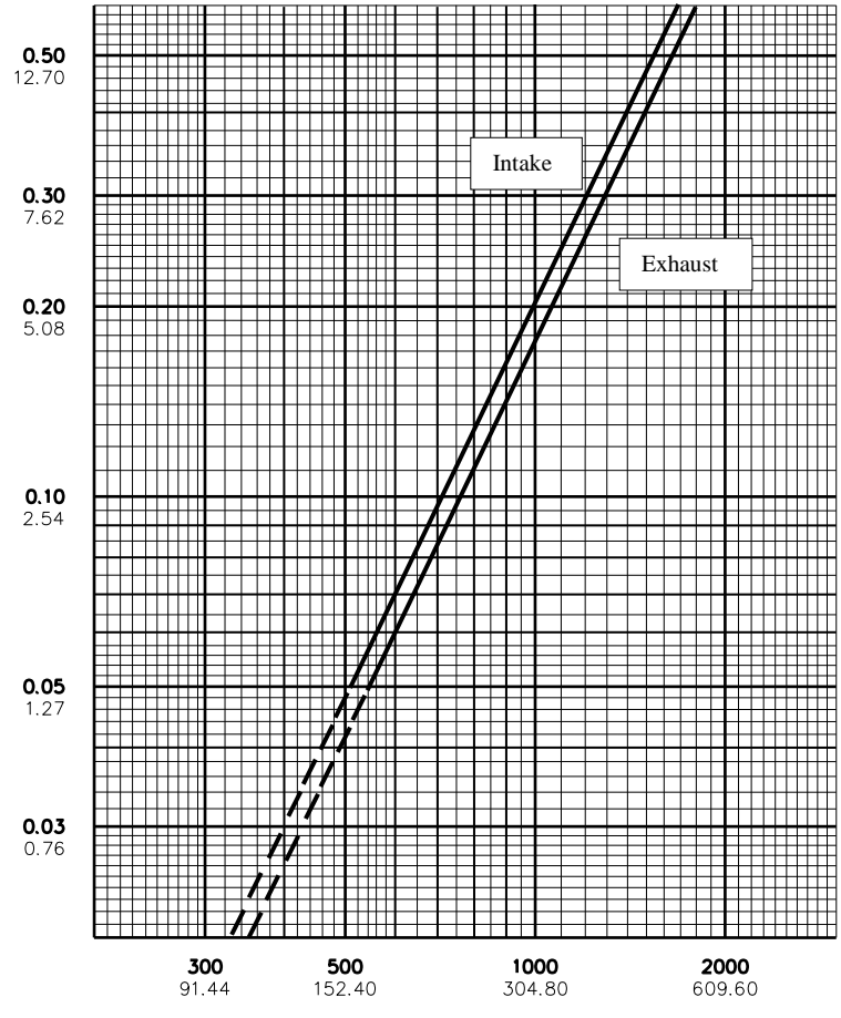
AIR VELOCITY IN FEET AND METERS PER MINUTE THROUGH FREE AREA For a 48" X 48" sized louver tested to figure 5.5. Data corrected to standard air density.
