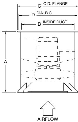
ARR. 4 – VERTICAL
