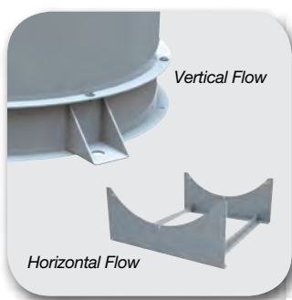
Support Legs
