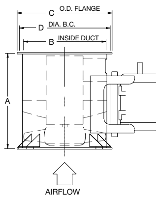
ARR. 9 – VERTICAL
