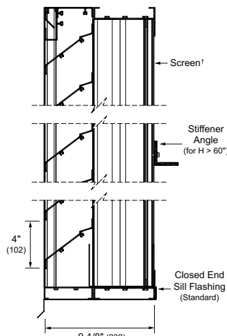
Vertical Section
