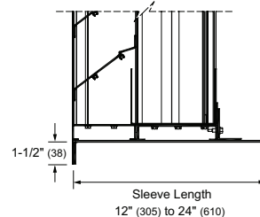
Sleeve (optional)
