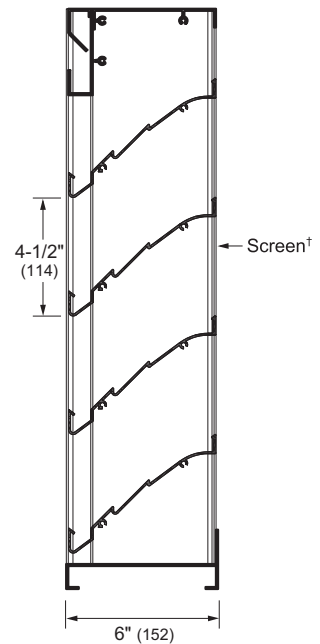
Vertical Section
