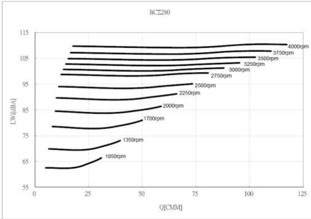
Sound Power [dB Ref 10-12 watts] %POF=( CMM*3531.5 / RPM x 1.03 )
