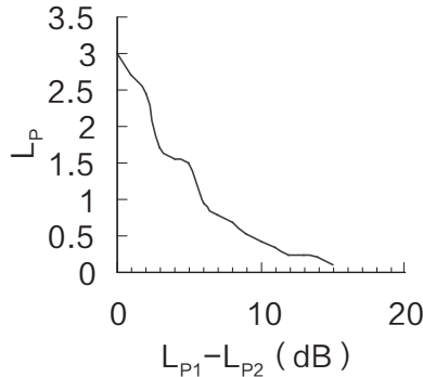
图 1 两噪声源的叠加曲线 Fig 1. Two noise sources superimposed curve
