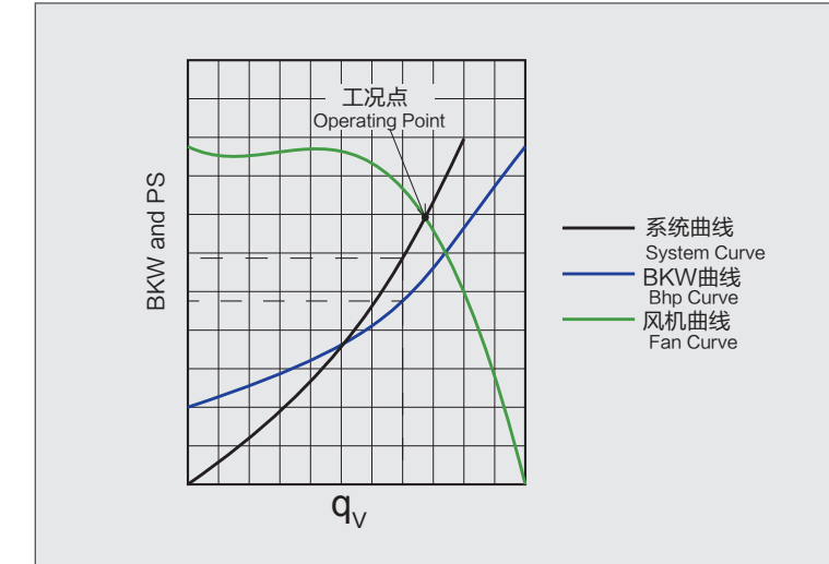
Fig.4 Operating Point
