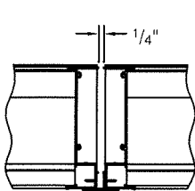
Standard Exposed Vertical Mullion (Available for NOA No: 05-1206.03)
