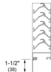
Flange Frame (optional)
