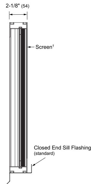
Vertical Section
