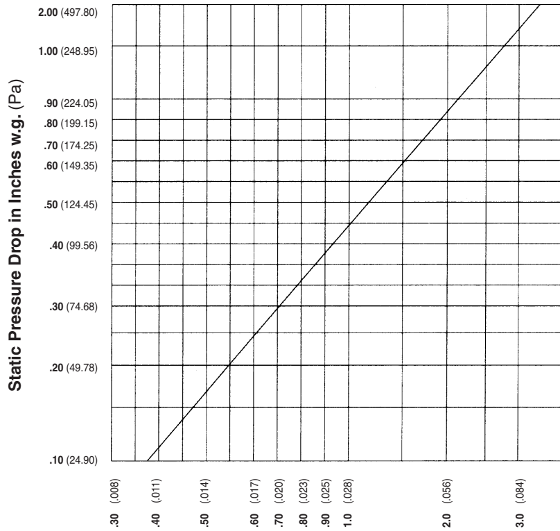
CFM (m³min.) Leakage per ft.² (m²) of Free Area
