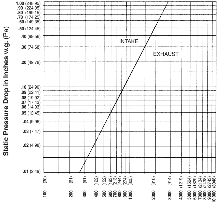
Air Velocity in feet (meters) per minute through Free Area (Data corrected to standard air density and AMCA figure or figures tested to 5.5)
