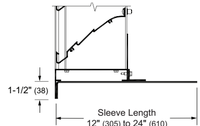
Sleeve (optional, single sections only)
