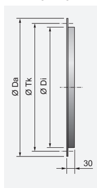
Matching flange
