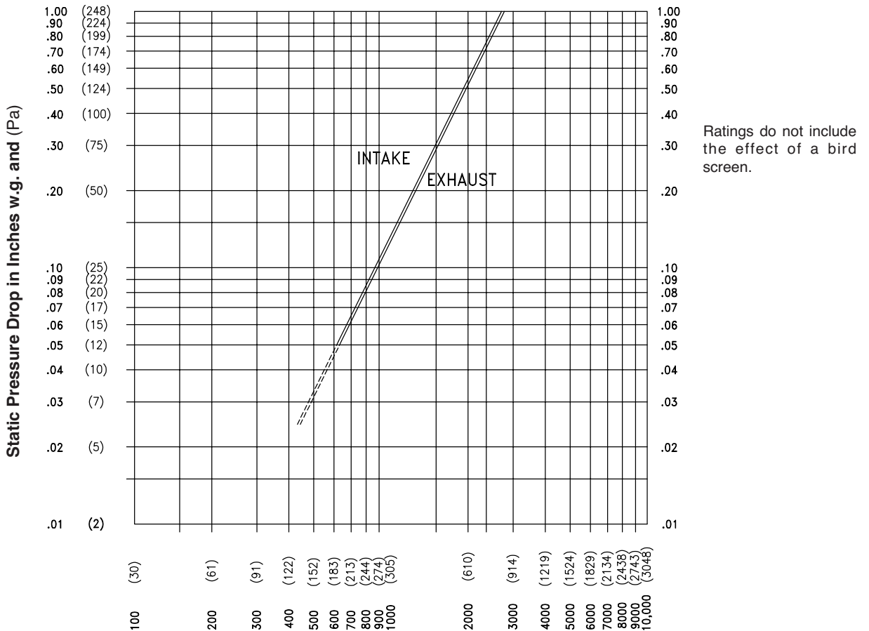
Air Velocity in feet and (meters) per minute through Free Area (Data corrected to standard air density and AMCA figure or figures tested to 5.5)
