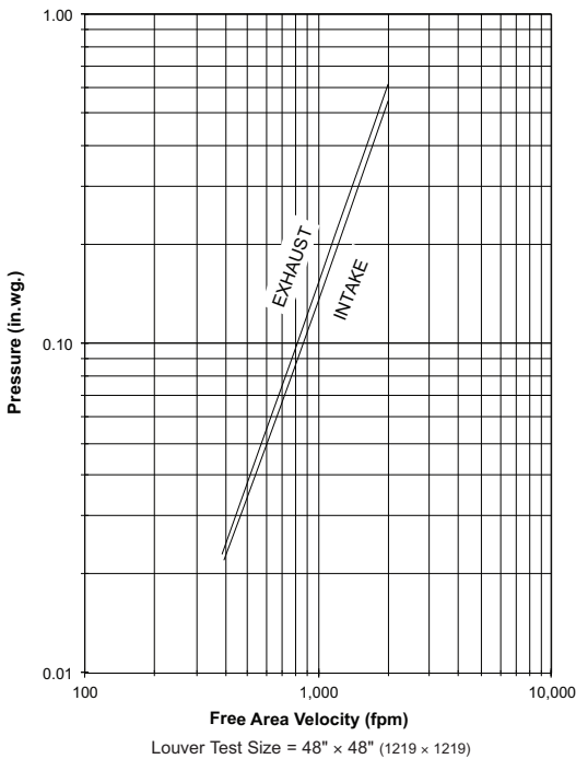
Pressure loss tested in accordance with Figure 5.5 of AMCA Standard 500-L.
