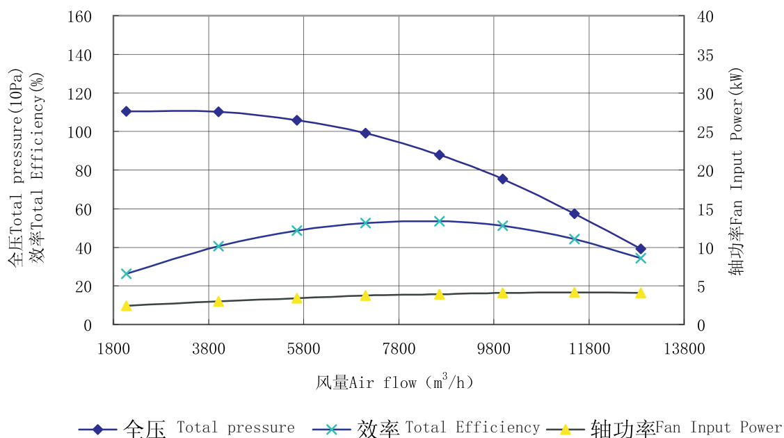
4-79-6A性能曲线图 (Performance curve) n=1450r/min
