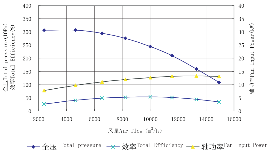
4-79-5A性能曲线图 (Performance curve) n=2900r/min
