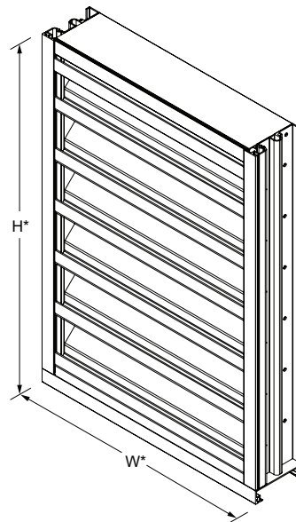
Model EFD-445 (standard) *Louver dimensions furnished approximately 1/2" (13) undersize.
