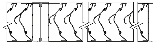
Vertical Mullion (standard)
