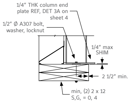
1. SILL DETAIL - WOOD SUBSTRATE (HEAD SIM) N.T.S. Ref Detail 2A/9, 2B/10, 2C/11, 2H/12 for alternate substrate materials
