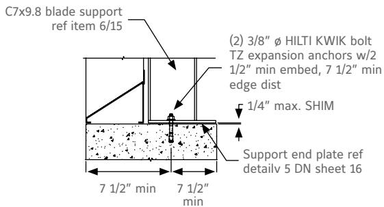
3. SUPPORT ATTACHMENT - CONCRETE SLAB N.T.S. 3000 psi. min concrete note edge requirements
