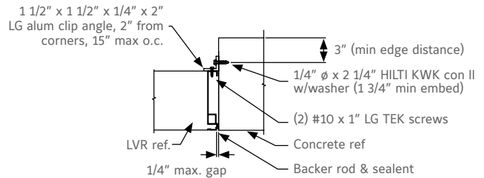
4. JAMB DETAIL - CONCRETE N.T.S. 3000 min compressive strength note edge distance requirements
