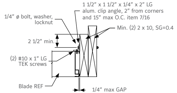
2. JAMB DETAIL - WOOD SUBSTRATE N.T.S. Ref Detail 1A/6, 1B/6, 1C/7, 1D/7, 1E/8 for alternate frame materials
