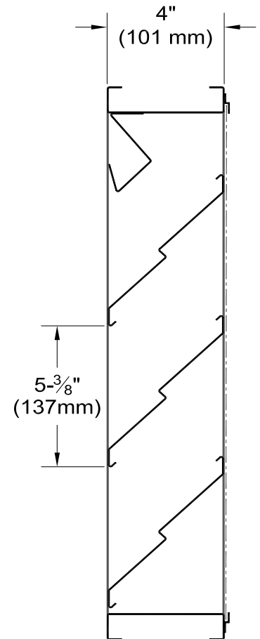
Channel Frame
