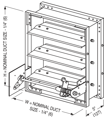
MODEL D1200 1 1/2 HOUR LABEL MODEL D1200-3 3 HOUR LABEL (Side Mounting Plate/Sleeve not shown)
