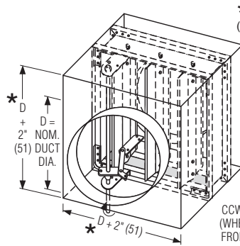
STYLE CR : FOR ROUND DUCT
