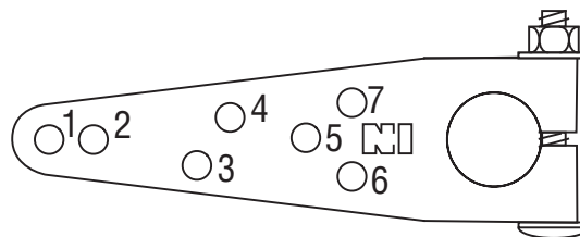
1" (25) DIA. CRANK ARM PART NO. CD010
