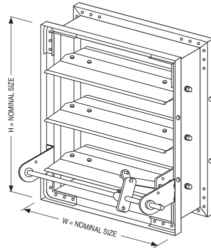
MODEL 1221-OW 1 1/2 HOUR LABEL (Sleeve not shown)
