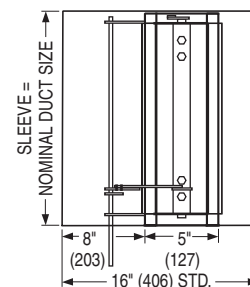
MODEL 1221VB: TYPE A SLEEVE
