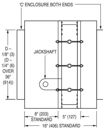
STYLE CR : FOR ROUND DUCT
