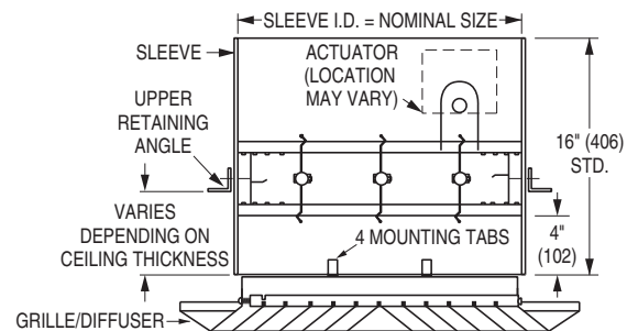
MODEL 1271C-1 (for use with Steel Grille/Diffuser)
