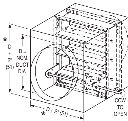
STYLE CR : FOR ROUND DUCT
