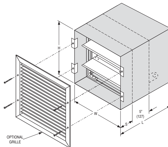
MODEL 1221G 1 1/2 HOUR LABEL
