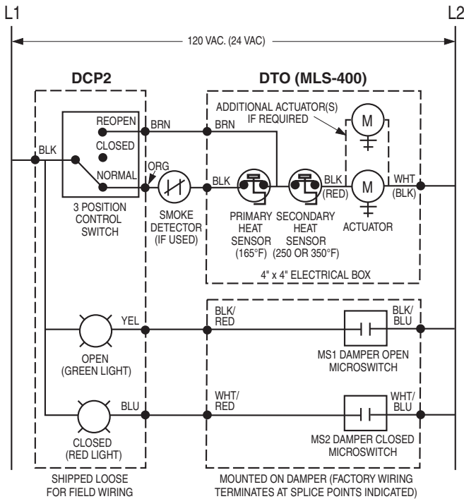
DCP2/DTO (MLS-400) with Honeywell rotary cam type position indicator package
