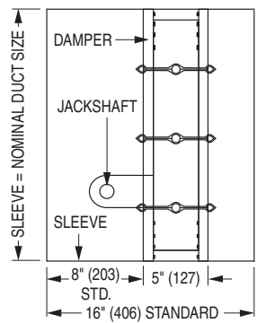
MODEL 1211BAL: TYPE A SLEEVE
