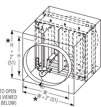
STYLE CSR : FOR SQUARE OR RECTANGULAR DUCT
