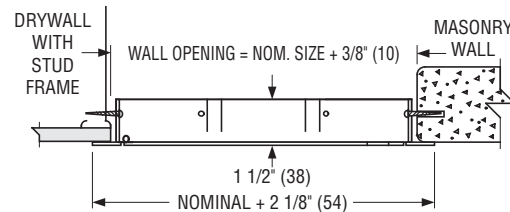
INSTALLATION DETAIL
