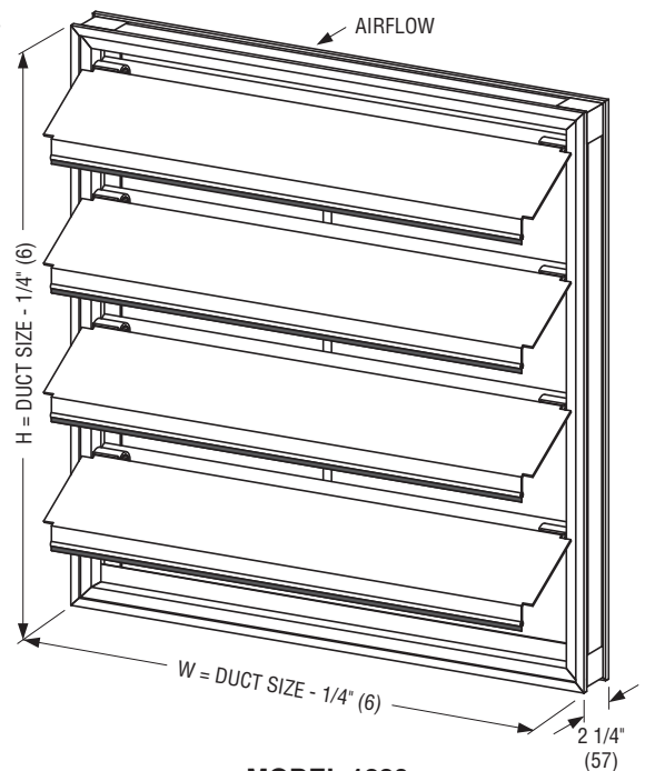
MODEL 1380 (VM Vertical Mount standard)
