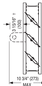
MODEL 1110 PARALLEL BLADE
