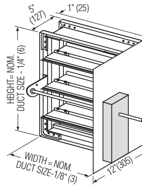
SIDE ACTUATOR MOUNTING PLATE FOR JACKSHAFT DRIVE
