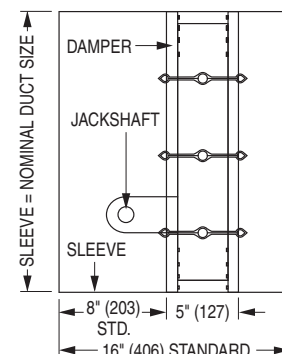
MODEL 1211M: TYPE A SLEEVE
