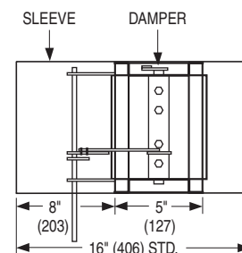
MODEL 1211VB: TYPE A SLEEVE
