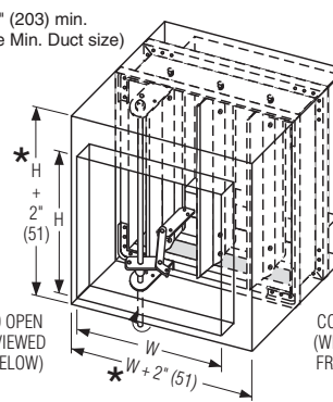
STYLE CO : FOR OVAL DUCT
