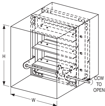
Models 1220BAL (no sleeve), 1221BAL, 1220BAL-3 (no sleeve) & 1221BAL-3 Sizes (Duct W x H):
