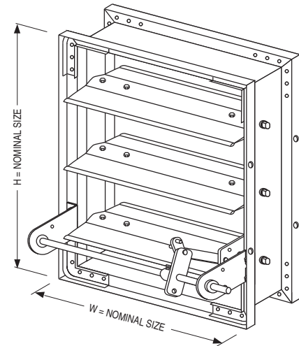
MODEL 1221-DOW 1 1/2 HOUR LABEL (Sleeve not shown)
