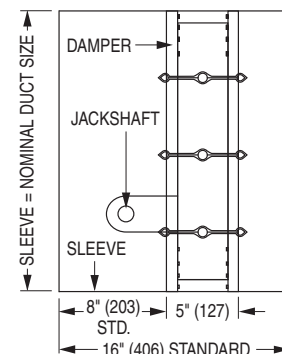
MODEL 1211SS: TYPE A SLEEVE
