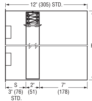
MODEL 0210G: TYPE A
