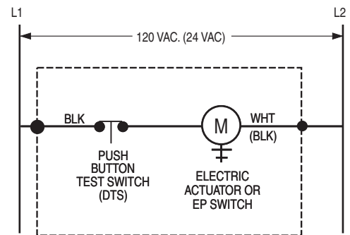
DTS Damper Test Switch
