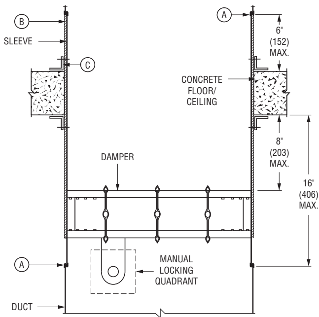
BELOW FLOOR INSTALLATION
