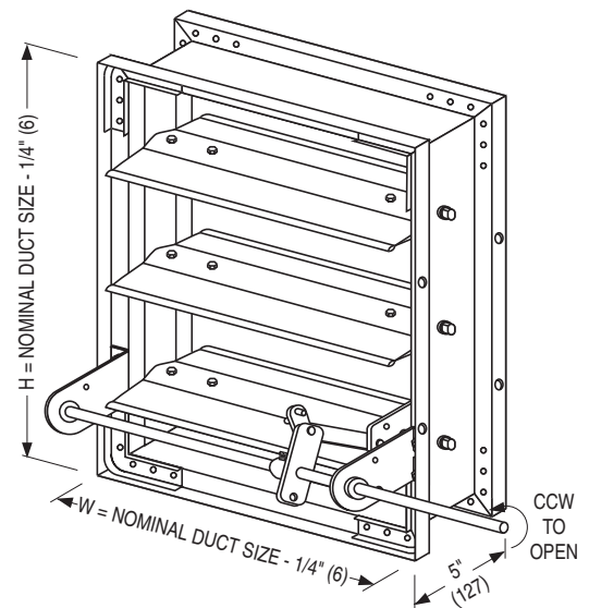
MODEL 1210M (Side Mounting Plate/Sleeve not shown)
