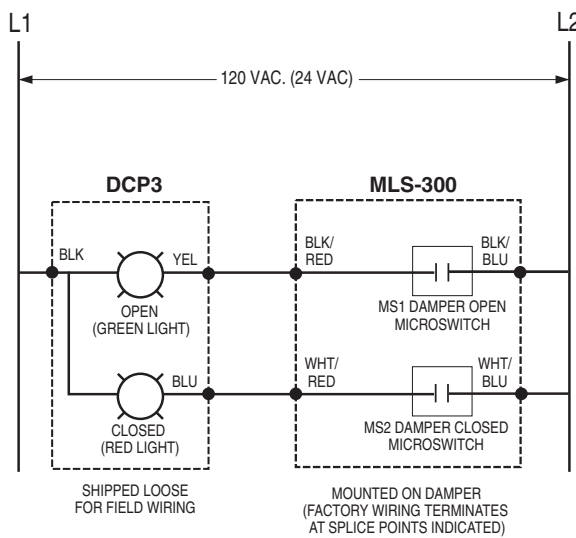
DCP3 with MLS-300 (Honeywell rotary cam type) position indicator package
