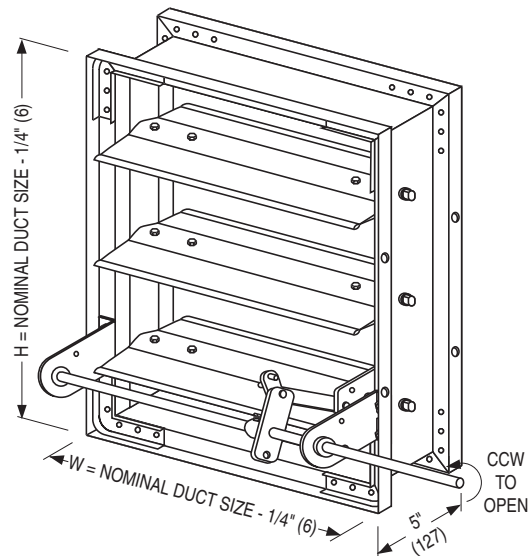
MODEL 1210BAL (Side Mounting Plate/Sleeve not shown)
