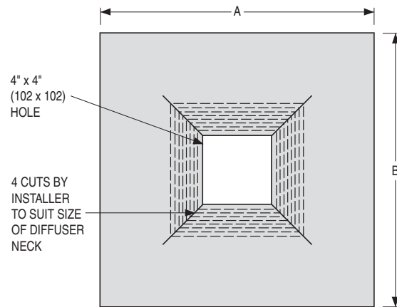
Model 0726: For square applications
