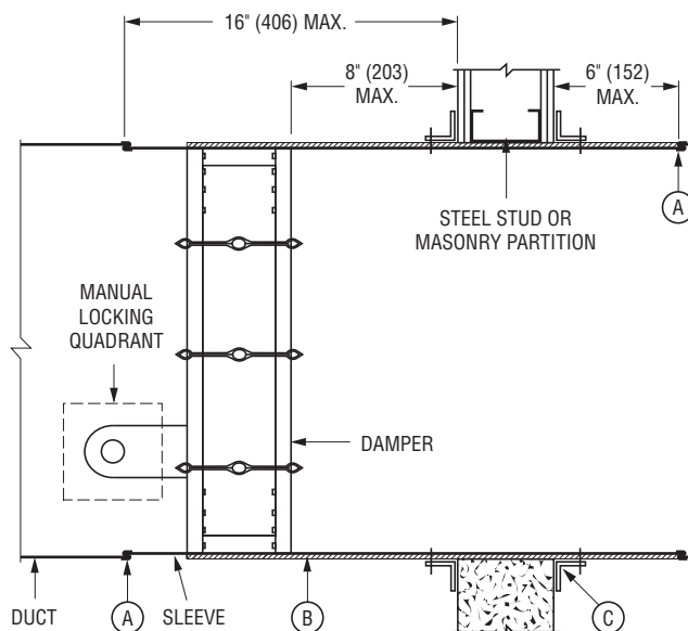
VERTICAL INSTALLATION
