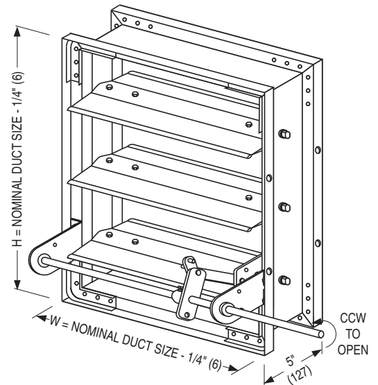
MODEL 1220BAL 1 1/2 HOUR LABEL MODEL 1220BAL-3 3 HOUR LABEL (Side Mounting Plate/Sleeve not shown)
