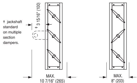
MODEL 2010-EAF PARALLEL BLADE
