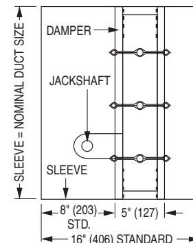
MODEL 1211: TYPE A SLEEVE
