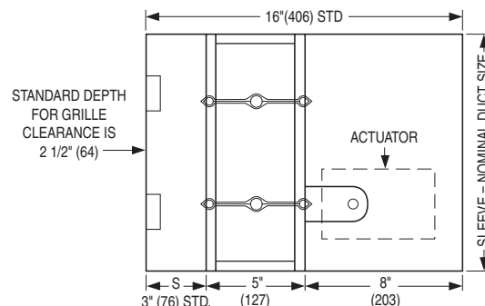
MODEL 1221G 1 1/2 HOUR LABEL
