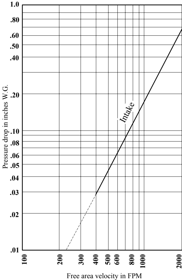
Air Performance
