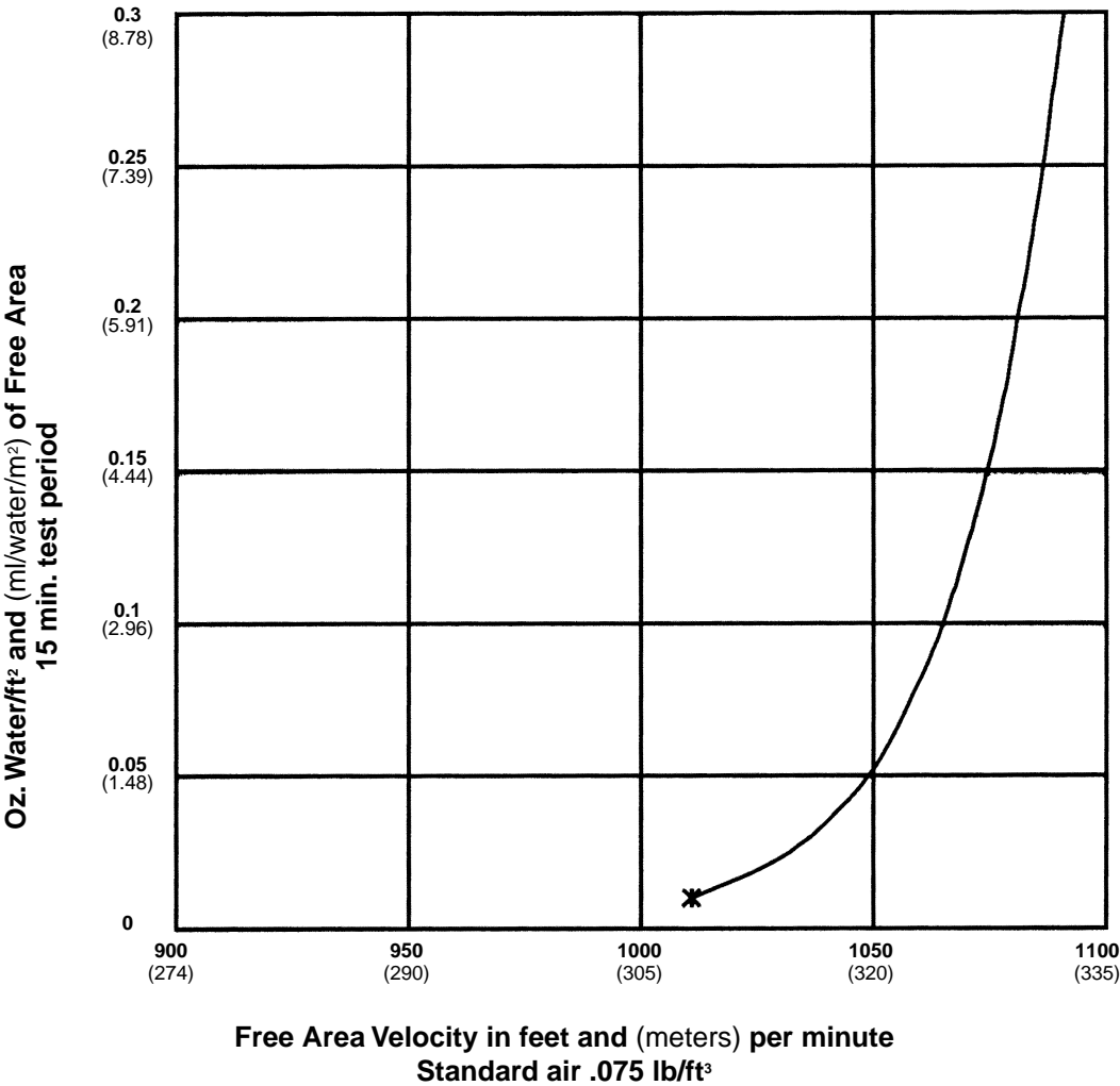
WATER PENETRATION Test size 48" wide x 48" high (1219 x 1219) Beginning point of water penetration at .01 oz./sq. ft. is 1010 fpm (308 m/min).
