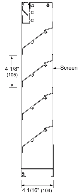
Vertical Section †Screen adds approximately 3/16" (5) to louver depth.
