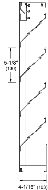
Vertical Section
