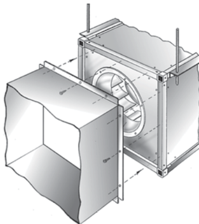
Mounting Frame Illustration
