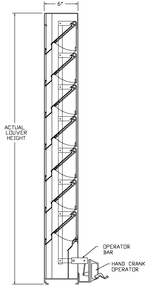
VERTICAL SECTION
